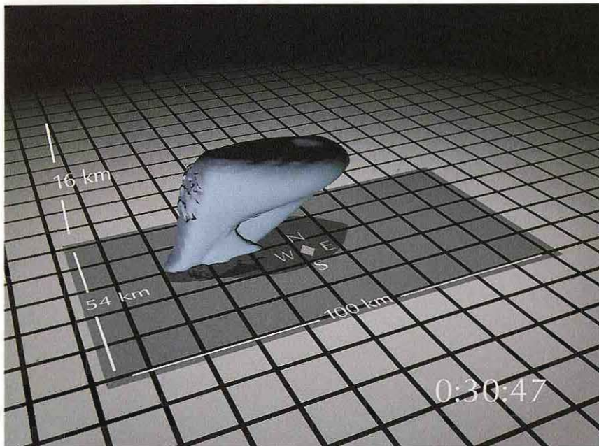
Image from the videotape "Study of a Numerically Modeled Severe Storm," National Center for Supercomputing Applications, University of Illinois at Urbana-Champaign, described in Robert B. Wilhelmson, Brian F. Jewett, Louis J. Wicker, Matthew Arrott, Colleen B. Bushell, Mark Bajuk, Jeffrey Thingvold, and Jeffery B. Yost, "A Study of the Evolution of a Numerically Modeled Severe Storm," International Journal of Supercomputer Applications , 4 (Summer 1990), pp. 20–36.
